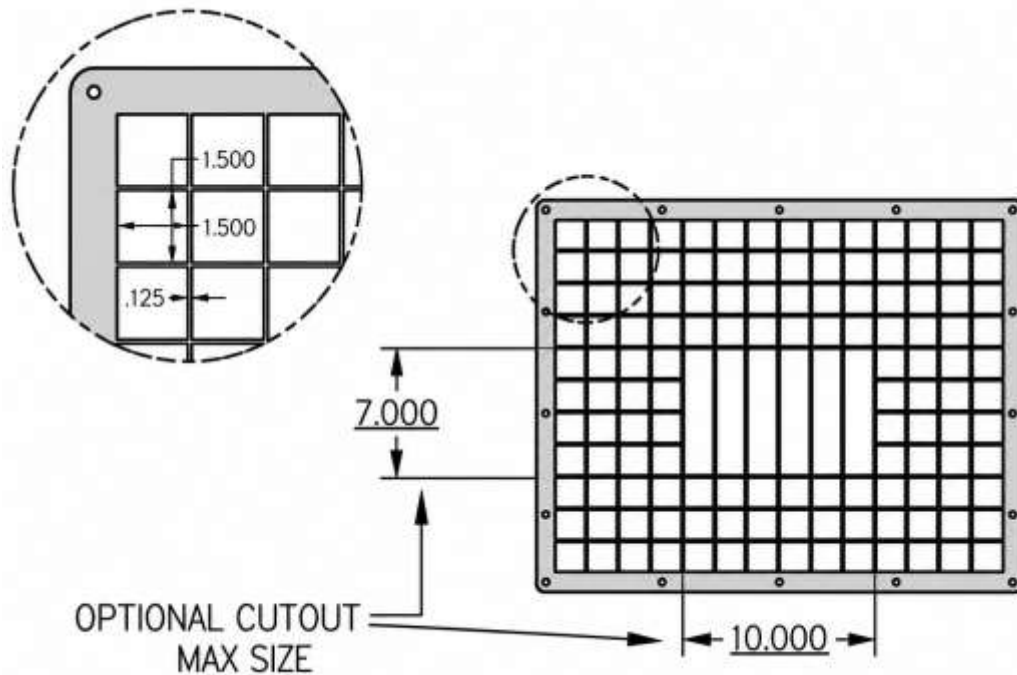
Figure 3 — Rock screen construction, opening size and optional cutout
