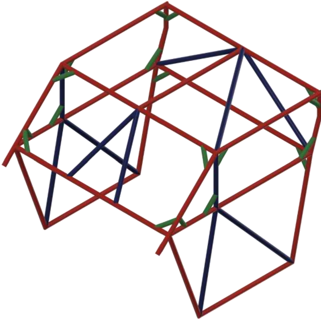
Figure 1 — General Roll Cage (All Classes), perspective view
